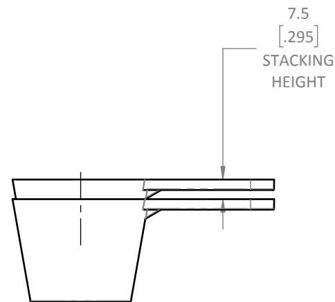
STACKING VIEW SCALE 1 : 2
